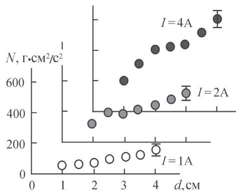
Fig. 2. Experimental values of the torque N exerted on the rotor of the MHD-motor at various depths of immersion d and strengths of direct current I.
