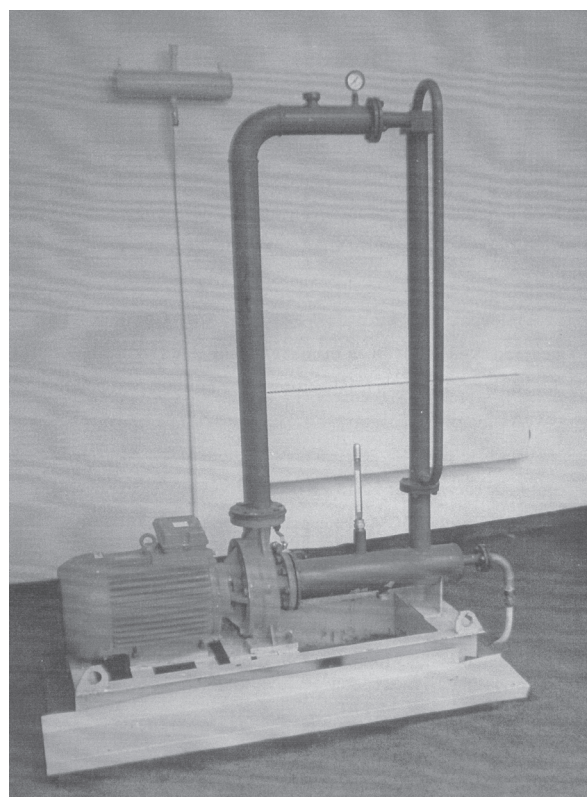
Fig.5 Heat generator
